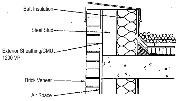
Roof At Parapet Wall
